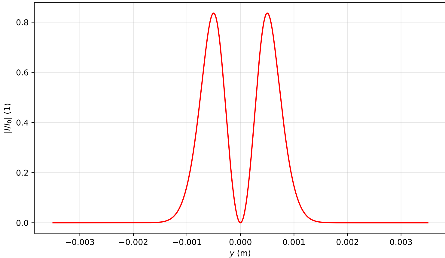
Intensity profile I(x=0, y, z=0.318)/I_0 , P_{in}=2.0P_{cr} , artificial time
